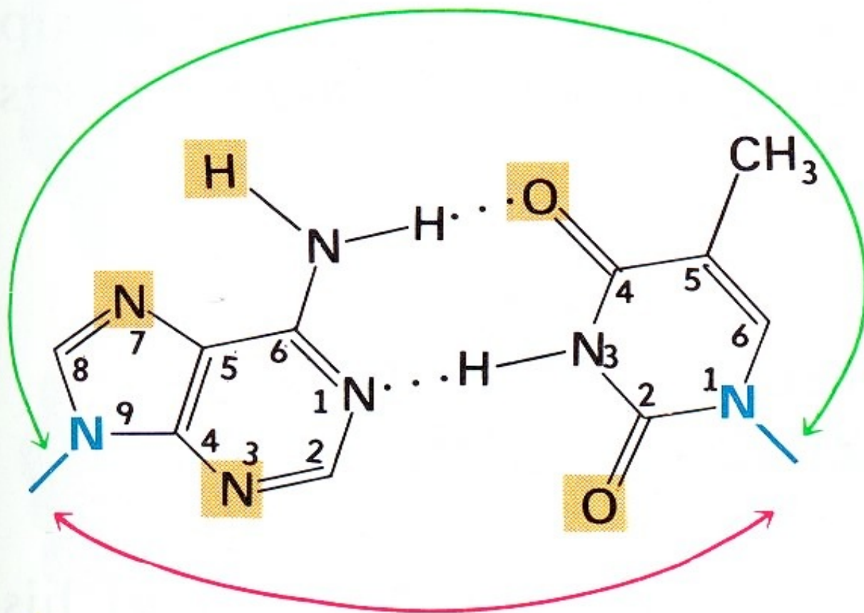
Minor groove
