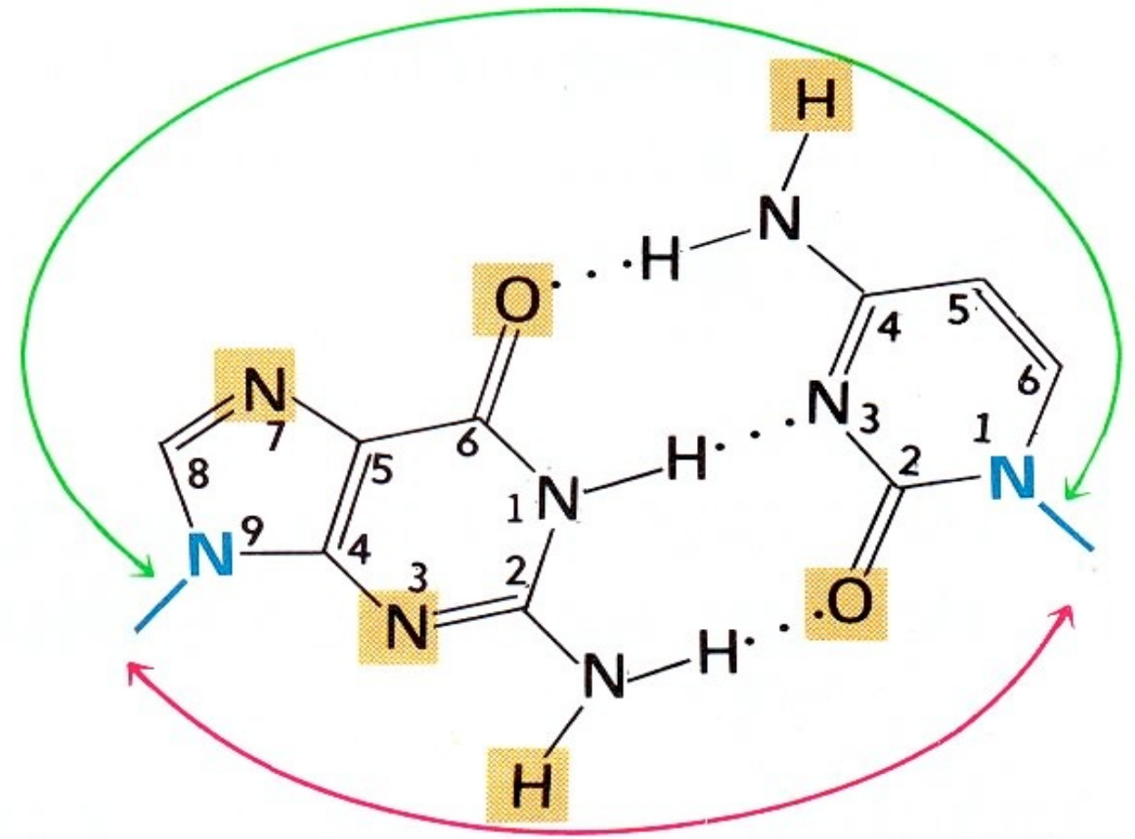
Minor groove
