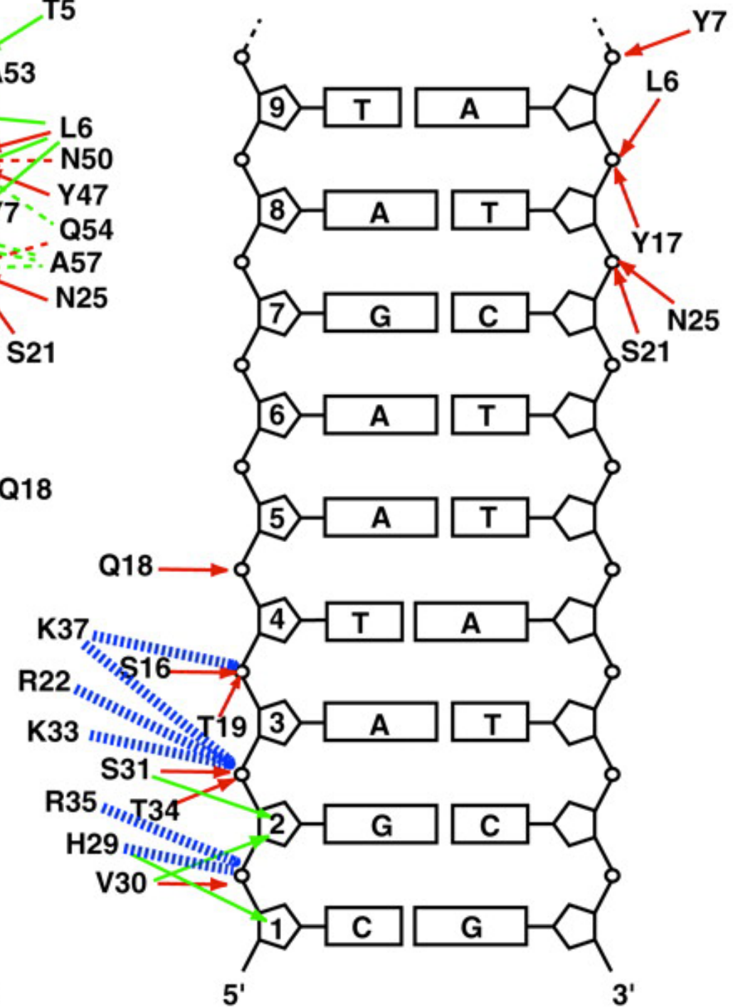
Non-specific complex
